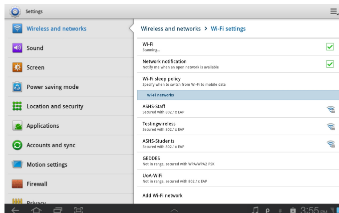
Figure 2: Select ASHS-Students
